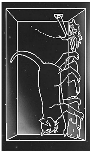
Schrödinger's Cat
