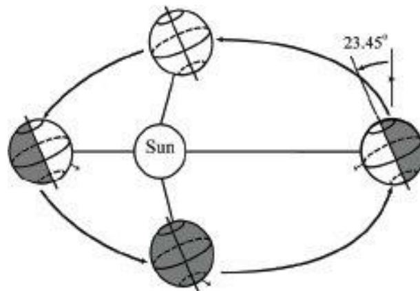
Fig. 96 – Earth orbit around the sun
