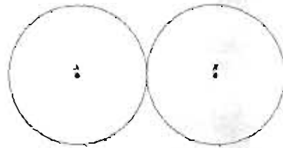
Figure 3 'Flatness' Hypersphere
