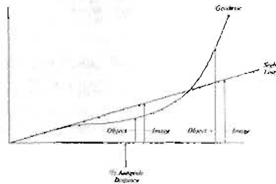
Figure 5 Hyperspherical Lensing
