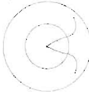
Figure 4 Geodesics in 'Flatness' Hypersphere
