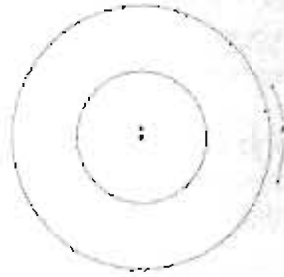
Figure 5 Hyperspherical Lensing
