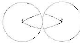
Figure 4 Geodesics in 'Flatness' Hypersphere
